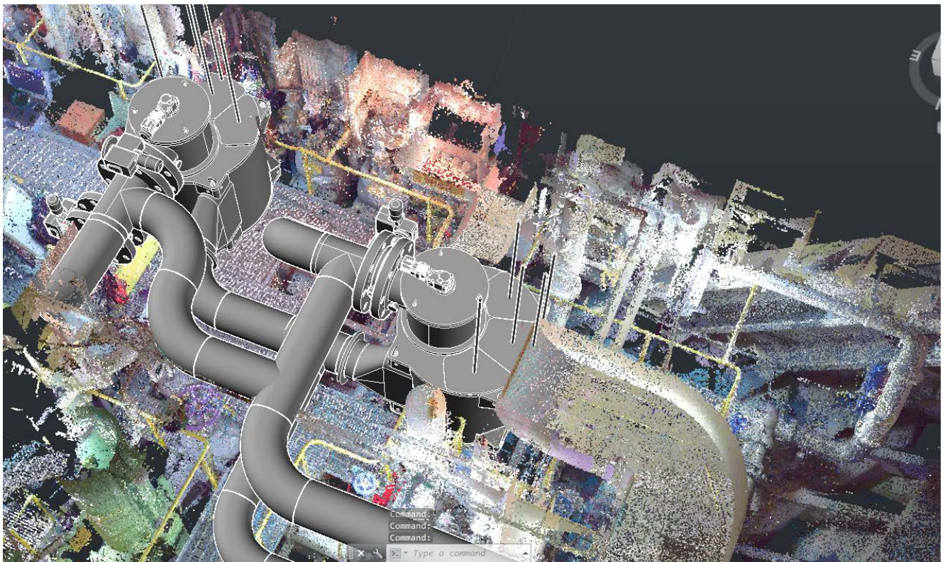
Picture 4: Set of Trojan Marinex fit & connected in vessel (using point cloud captured by other company)
